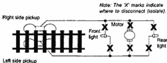
Figure 1. Connection of standard locomotive
