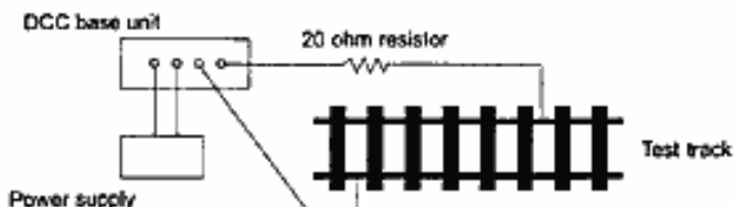
Figure 3. Diagram of test track
