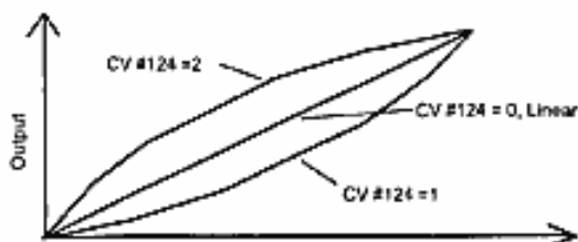
Speed curve of different value of CV #124
