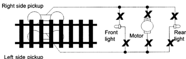
Figure 2. How to wire the decoder.
