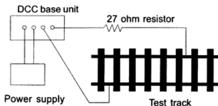
Figure 3. Diagram of test track
