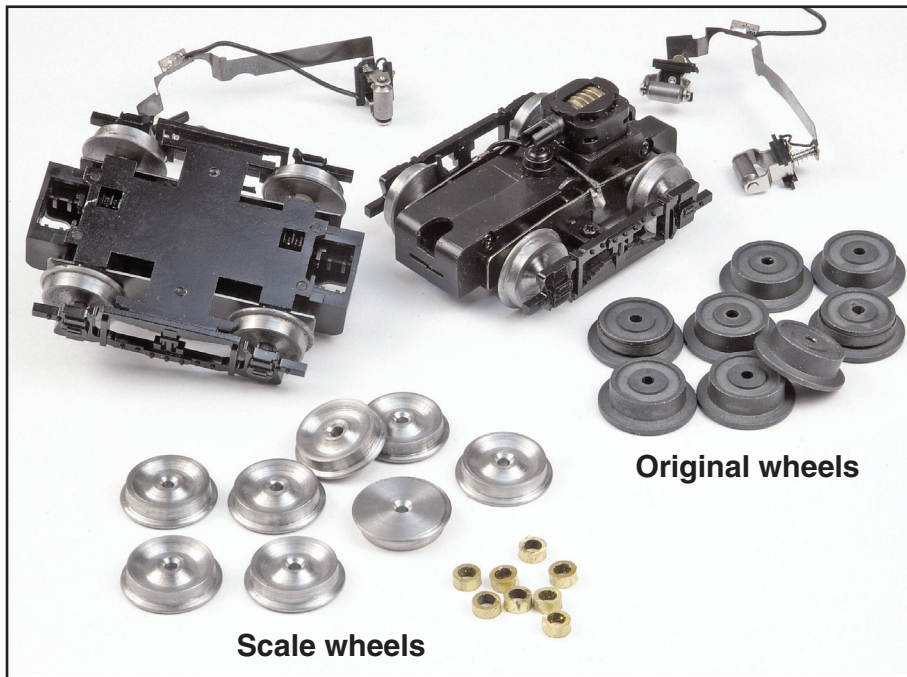
Scale wheels with axle bushings to reduce side-play in the trucks.
