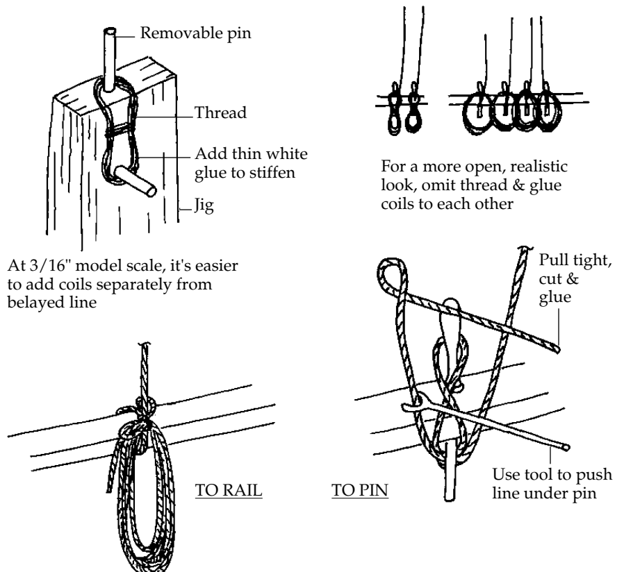
FIG. 55 - Rope Coils
