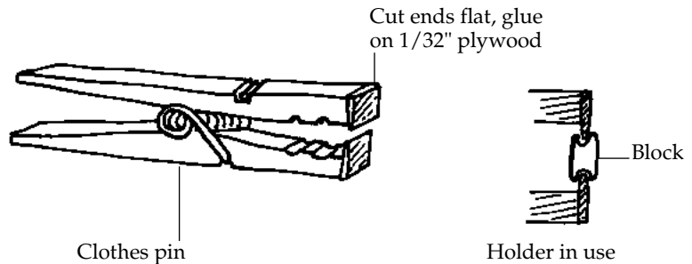
FIG. 57 - Block-holding Jig
