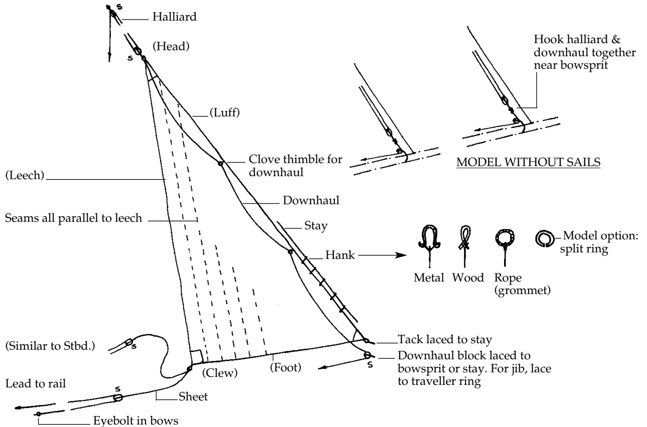
FIG. 70 -Typical Head Sail Rig
